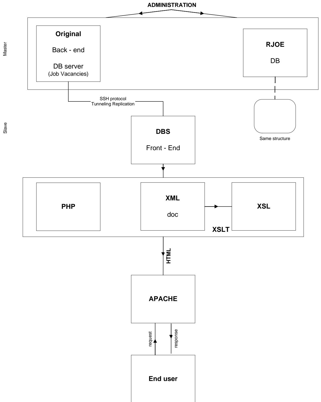
Figure 3. DB structure
