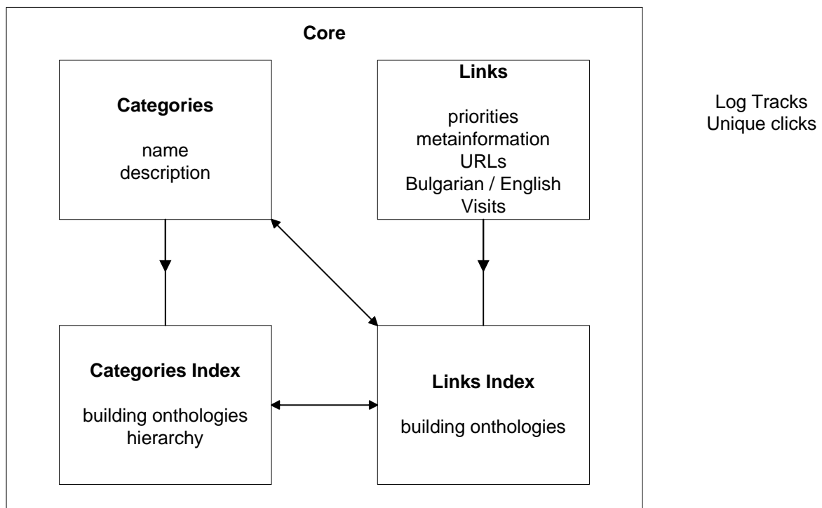
Figure 4. DB structure
